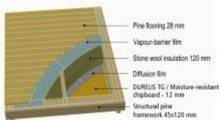
FLOOR STRUCTURE
